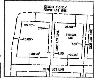
TYPICAL LOT SETBACK
